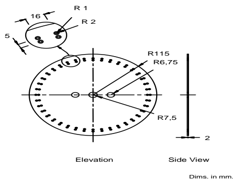
Fig. 1: Schematic diagram of the vertical grain plate.
