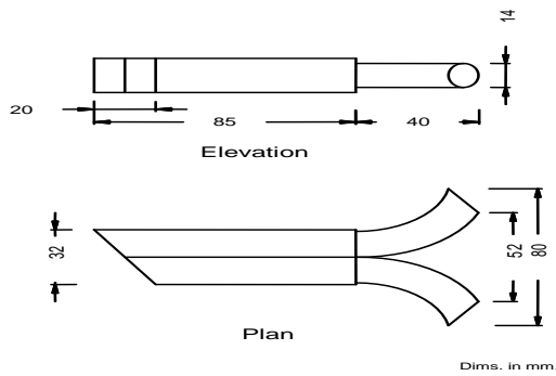
Fig.3: Grain delivery device
